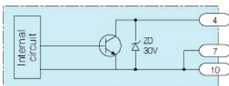
Open collector output (PS3F,PS3F-SR)
