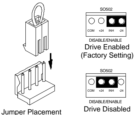
Figure 8. DISABLE/ENABLE Terminals
