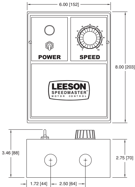
Figure 11. NEMA 1 Mounting Hole Locations
