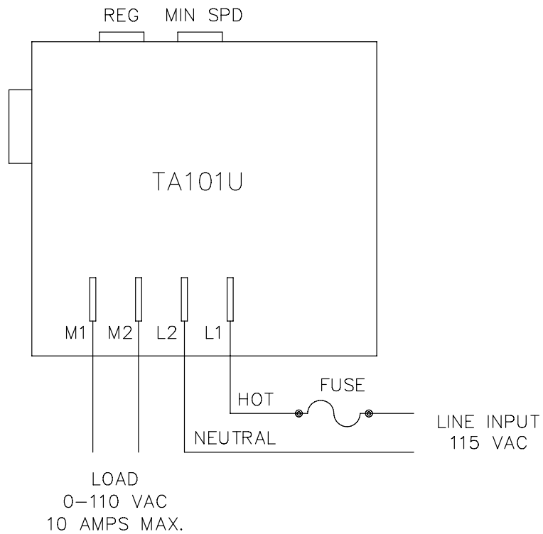
TA101U Connection Diagram
