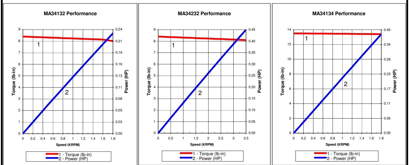
Curves: 1) Speed vs Torque Curves, 2) Output Power vs. Speed
