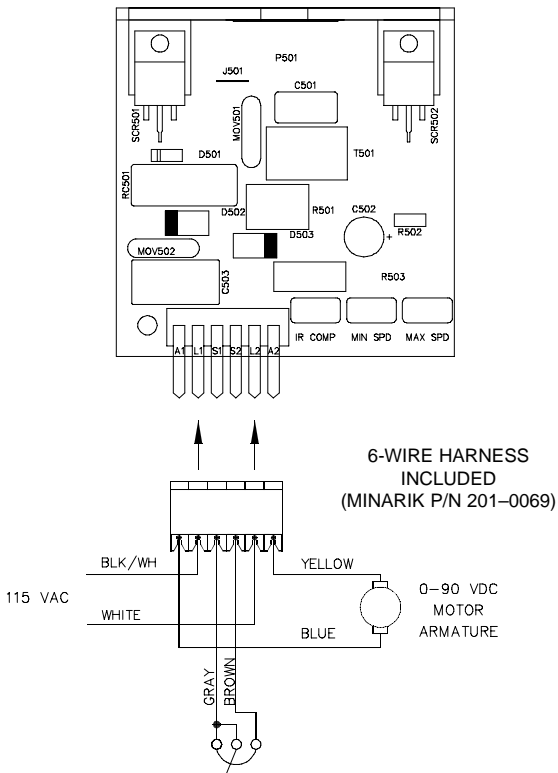
Figure 3. MM31700B/MM31701B Connections
