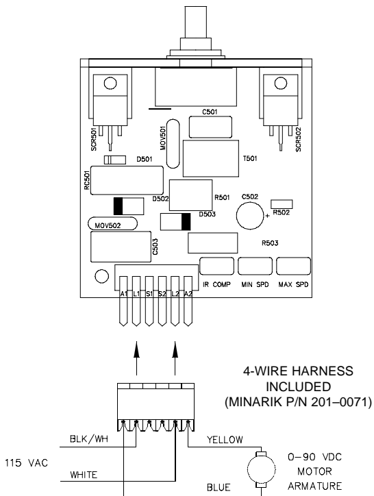
Figure 4. MM31750B/MM31751B Connections
