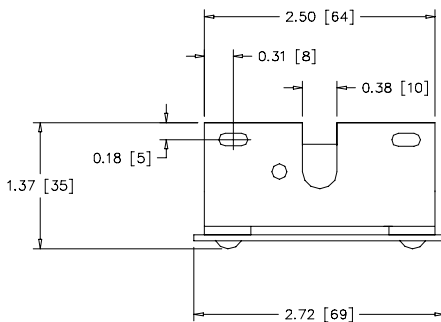
Figure 1. MM31700B/MM31701B Dimensions
