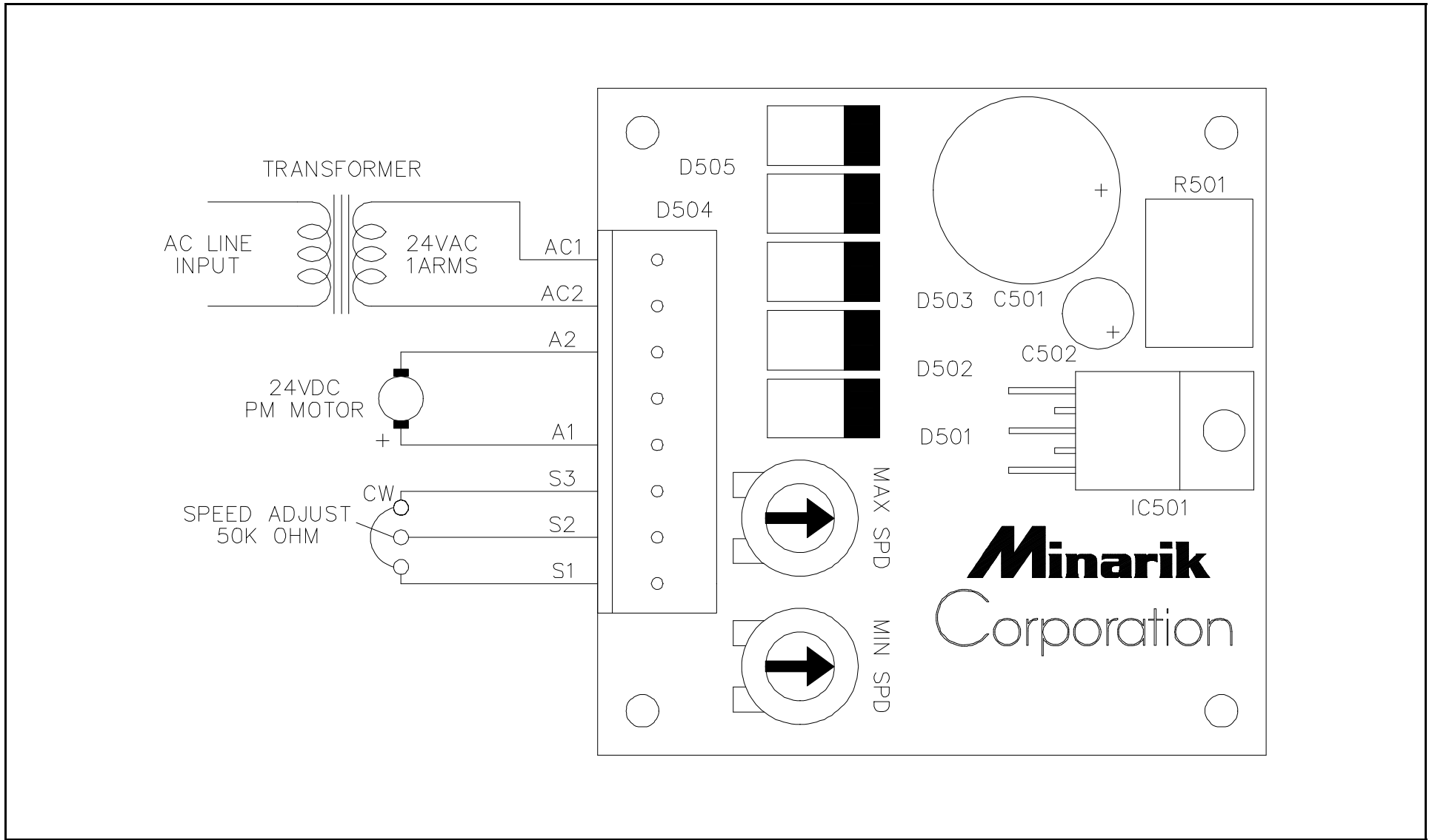
LV01-24AC-E10U Connection Diagram
