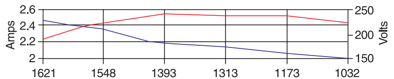
Variable speed graph for catalogue M099901 using a Norsol Vari-Vent control.
